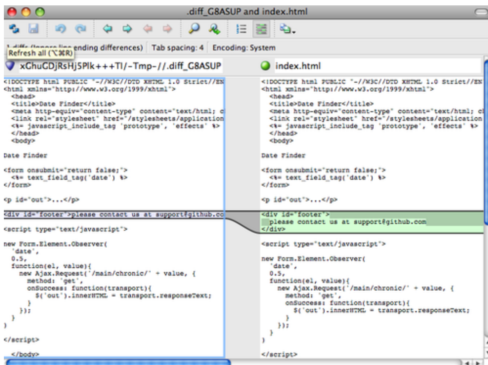
Figure 143. P4Merge.
